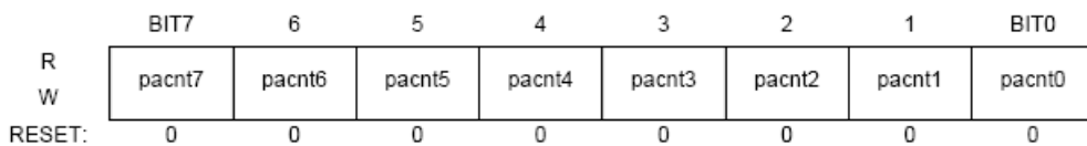
Figure 3-20 Pulse Accumulators Count Register 0 (PACN0)
