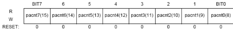
Figure 3-17 Pulse Accumulators Count Register 3 (PACN3)
