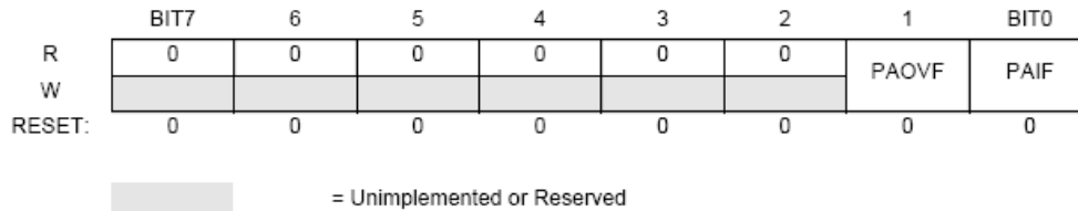
Figure 3-16 Pulse Accumulator A Flag Register (PAFLG)
