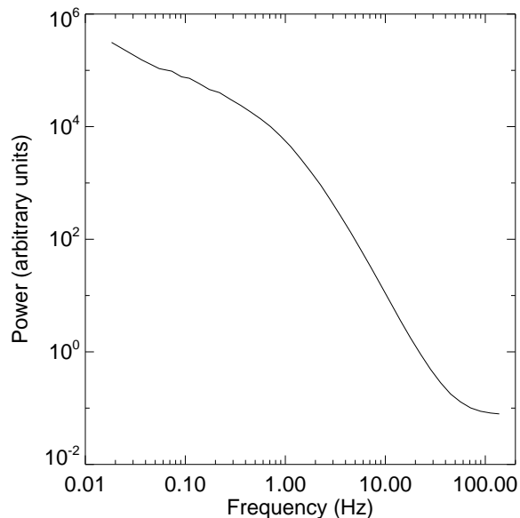
Fig. 10.— Power spectrum of the signal measured by a single sensor. Notice the break in the spectrum around 1 Hz, as well as the noise floor apparent above 30 Hz.
