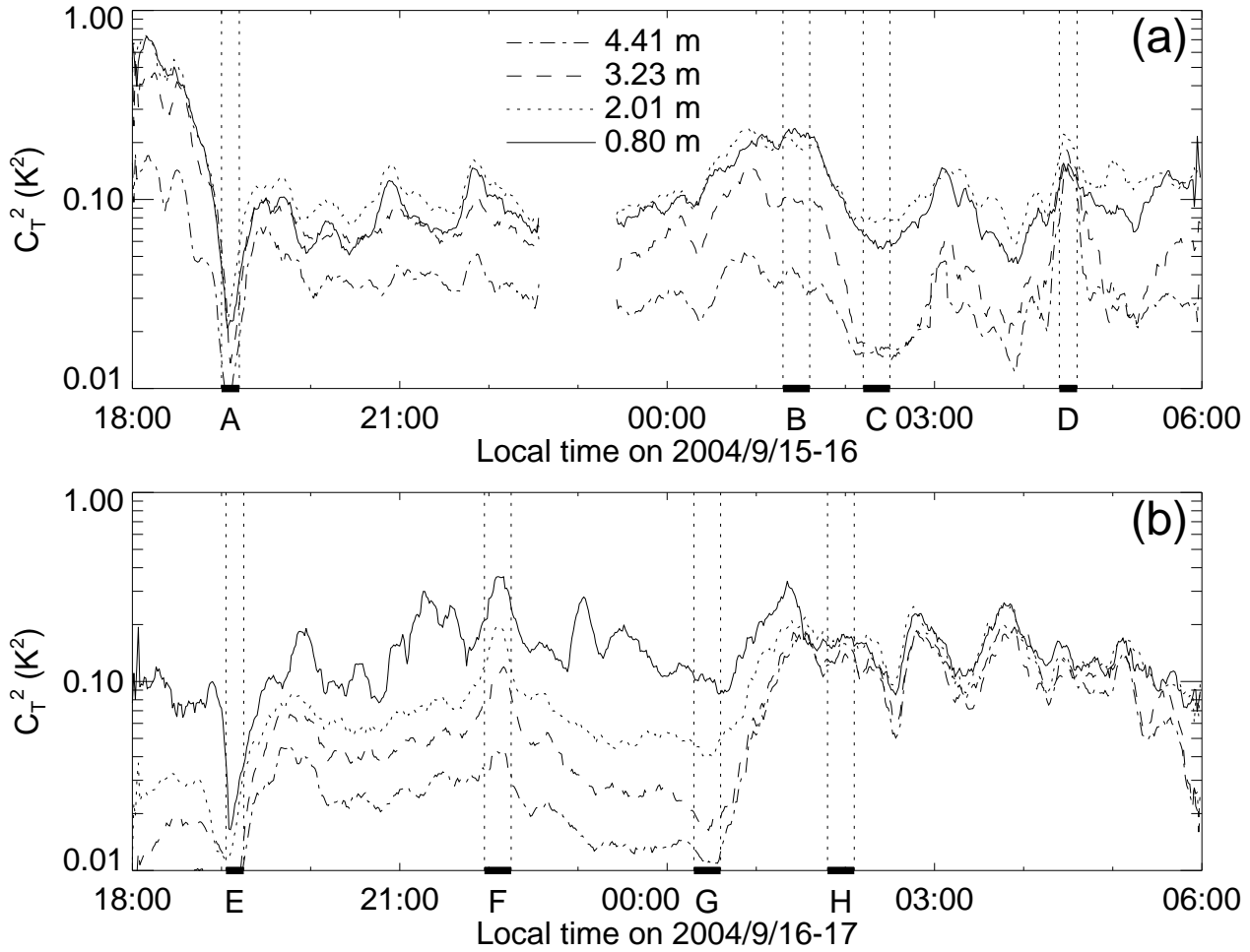
Fig. 8.— (a) C_T^2 for the four different sensor pair heights on (a) the night between September 15 and 16, and (b) the night between September 16 and 17. C_T^2 values have been smoothed with a 11-minute window to allow longer-term time-variations to stand out.
