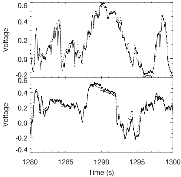
Fig. 4.— Verification of calibration by placing sensors very close together. Two sensor arms were placed facing each other such that the sensors in the two pairs were separated by less than 2 cm.
