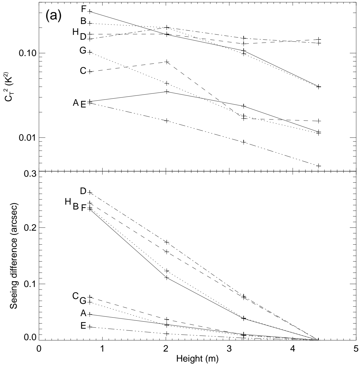
Fig. 9.— (a) C_T^2 as a function of altitude for the 8 intervals A through H labeled in Figure 8. (b) Computed seeing difference as a function of altitude, assuming a 1'' seeing at the top sensor.
