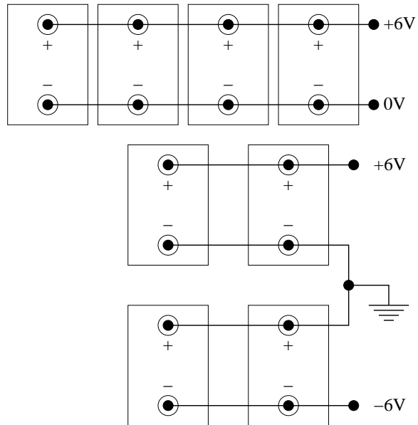
Fig. 3.— Schematic of the battery power system for the data acquisition and radio system, and for the sensor amplifiers.
