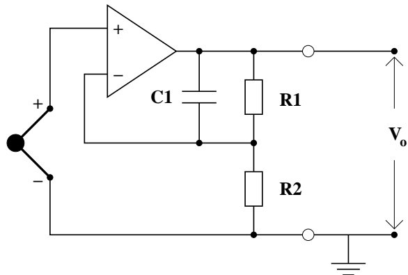
Fig. 2.— Schematic of the amplifier board. The thermocouple is shown to the left.
