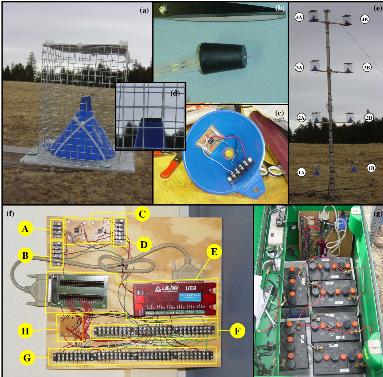
Fig. 1.— Photos of the hardware: (a) assembled sensor in the field, (b) insulated thermocouple mounted in plug, (c) inside of a sensor housing with amplifier board and external connector, (d) close-up of the thermocouple mounted at the top of the sensor assembly, (e) an entire tower, 15' tall, (f) data acquisition board [(A) 0-6V input power for UE9 and radio, (B) -6 - +6 V input for sensors amplifiers, (C) 5V voltage regulators for UE9 and radio, (D) 5V regulated outlet, (E) UE9 data acquisition unit and auxiliary input board, (F) sensor power distribution points, (G) sensor connections (there are four screws for each sensors, providing ground, positive and negative voltage for the amplifier, and return voltage measurement), (H) voltage monitoring board], (g) battery power system.
