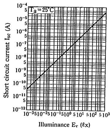
Fig. 1 Short Circuit Current vs. Illuminance
