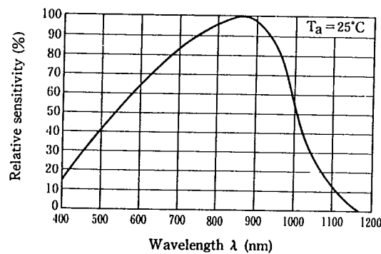
Fig. 4 Spectral Sensitivity
