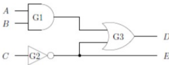
Figure 2: Simple Circuit
