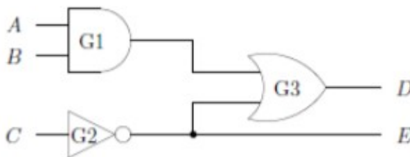
Figure 2: Simple Circuit
