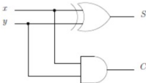
Figure 1: Half Adder Circuit
