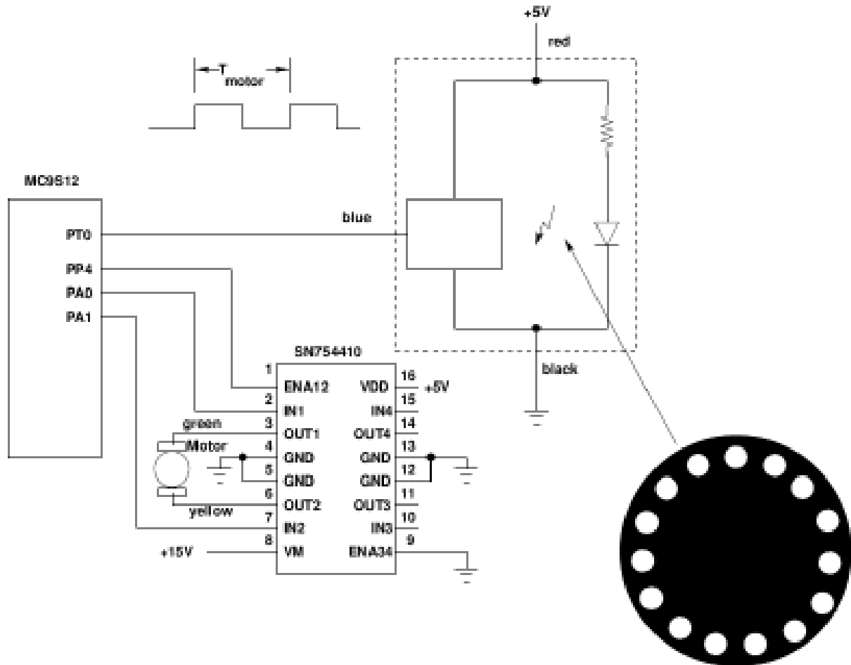
Figure 1: Using a PWM signal to adjust the speed of a motor.
