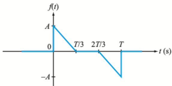
Figure P5.43: Waveform for Problem 5.43.
