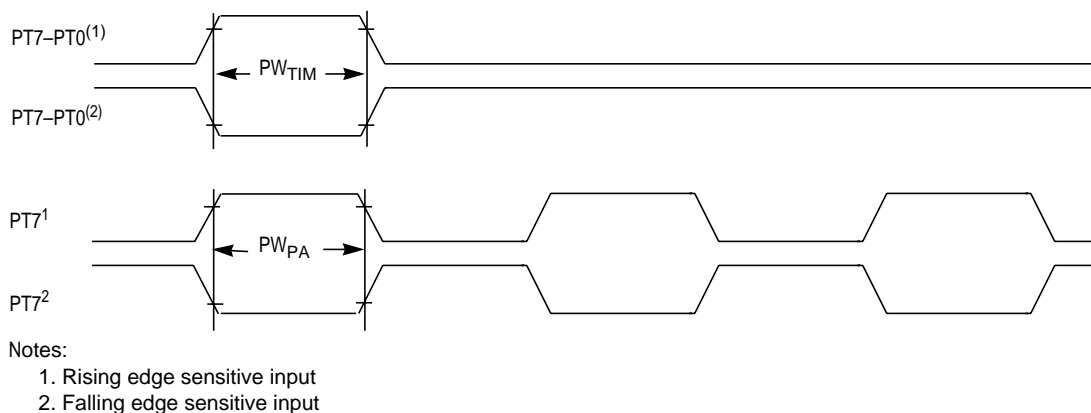
Figure 18-3. Timer Inputs
