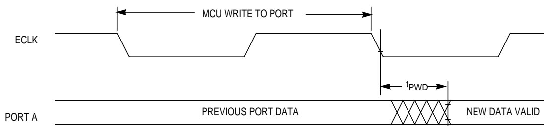
Figure 18-9. Port Write Timing Diagram
