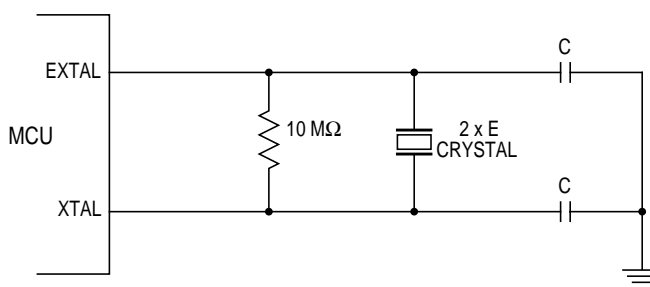
Figure 1-3. Common Crystal Connections
