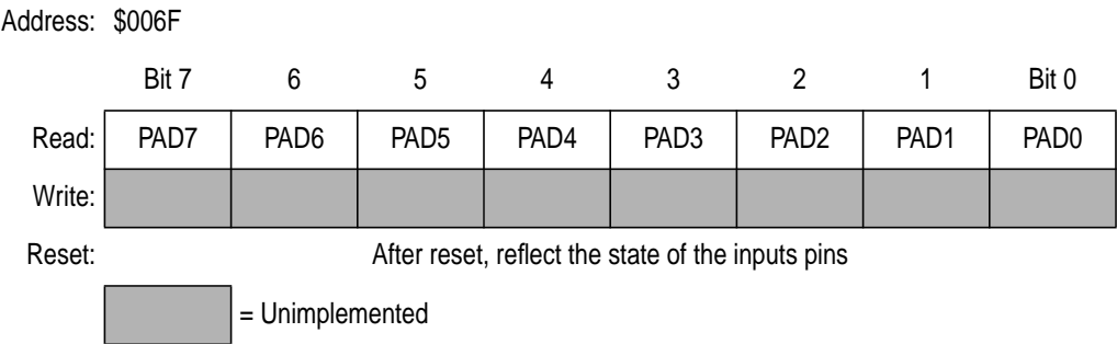
Figure 16-10. Port AD Data Input Register (PORTAD)
