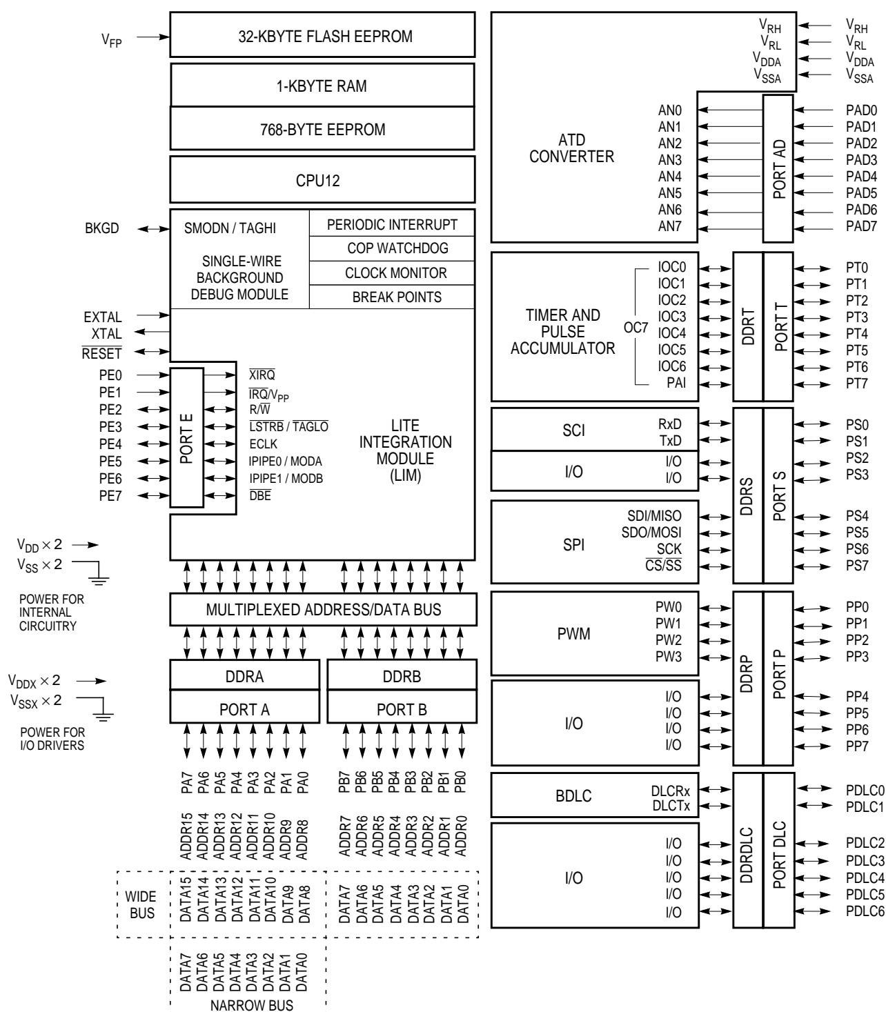
Figure 1-1. Block Diagram
