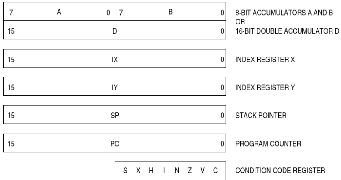
Figure 2-1. Programming Model
