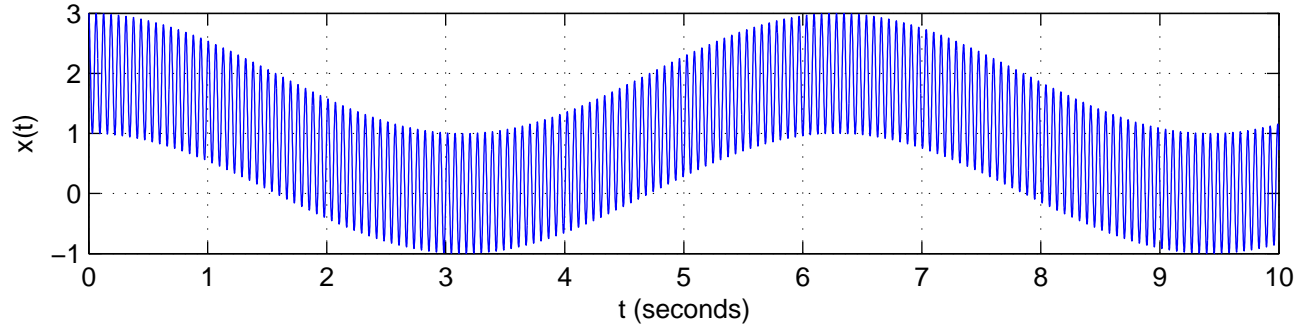
Effect of filter with H(\omega) = 10/(j\omega + 10)
