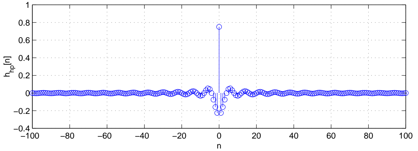
Truncated high-pass filter, 201 terms
