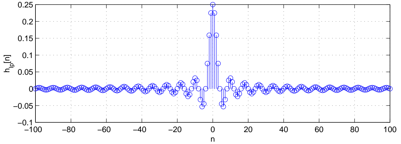
Truncated low-pass filter, 201 terms
