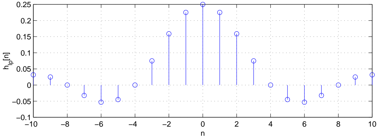
Truncated low-pass filter, 21 terms
