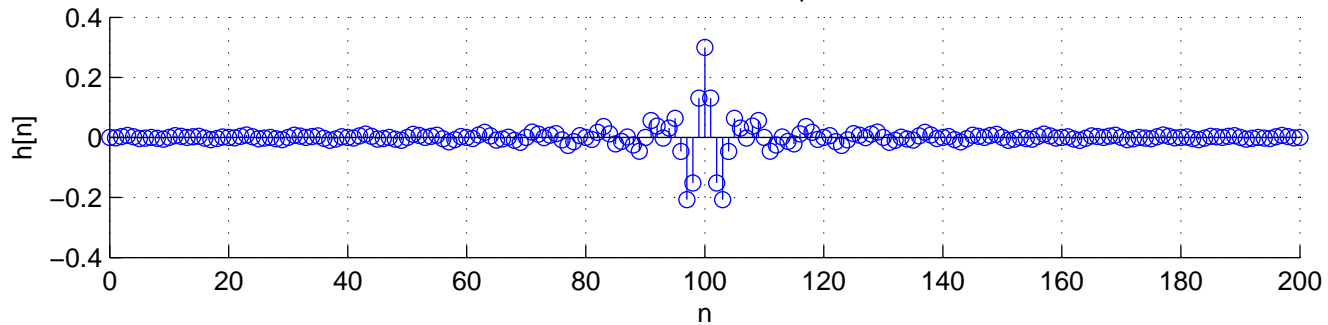
200 th causal order band-pass filter
