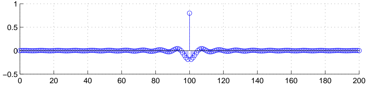
200 th causal order high-pass filter
