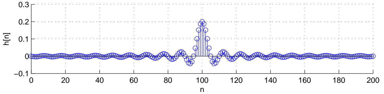
200 th causal order low-pass filter
