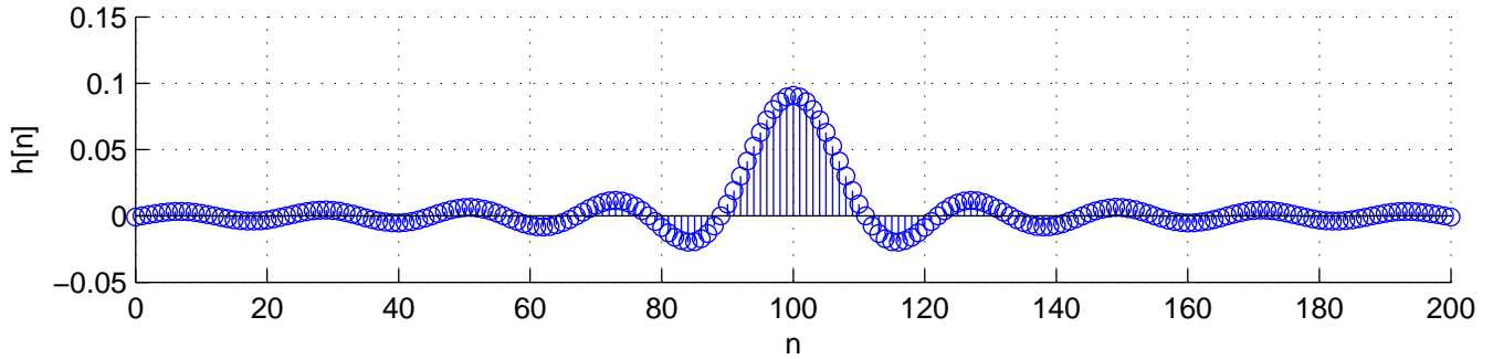
Low-pass filter, f_s = 44 \text{ kHz} , f_c = 2 \text{ kHz}
