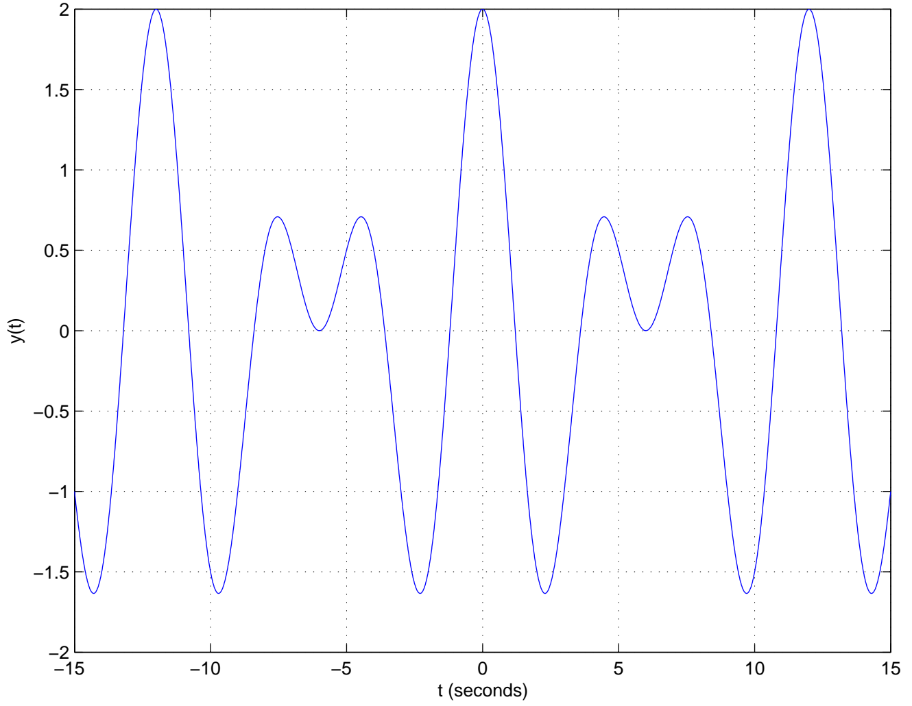
Plot of y(t) = \cos(\pi t/2) + \cos(\pi t/3)
