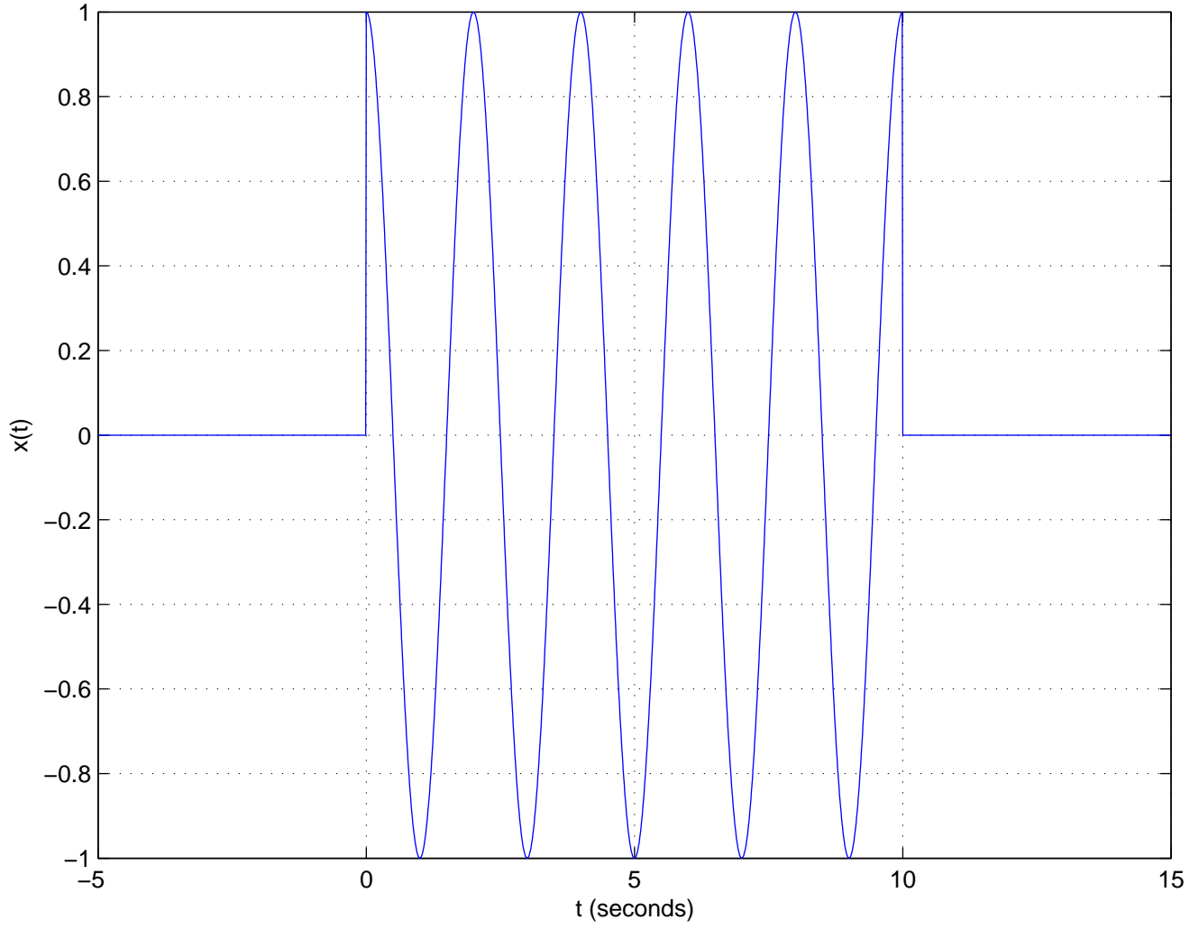
Plot of \cos(\pi t) (u(t) - u(t-10))
