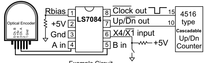
Example Circuit
